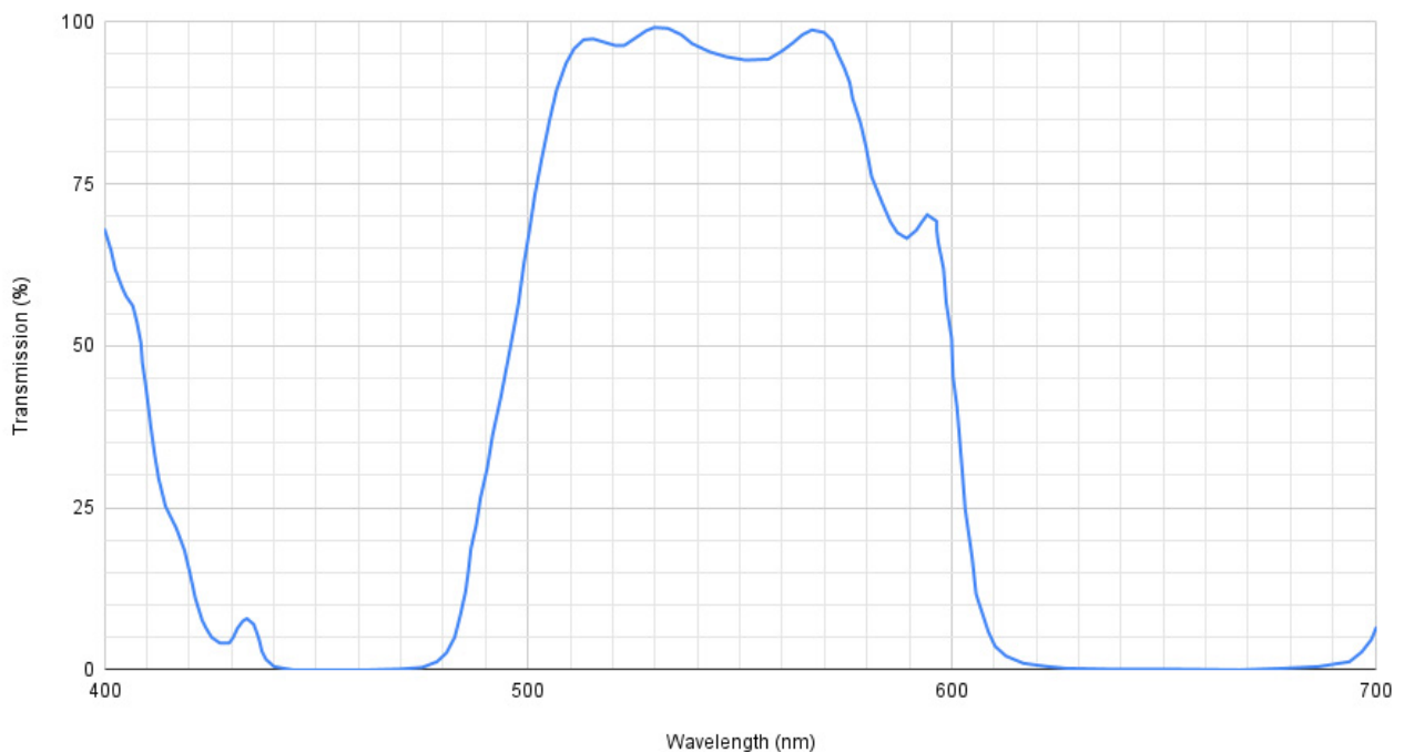
Dichroic Filter "refl. red/blue"
