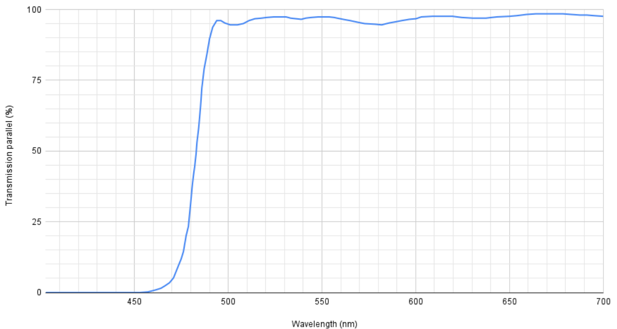
Dichroic Filter "refl. blue" (parallel, p)
