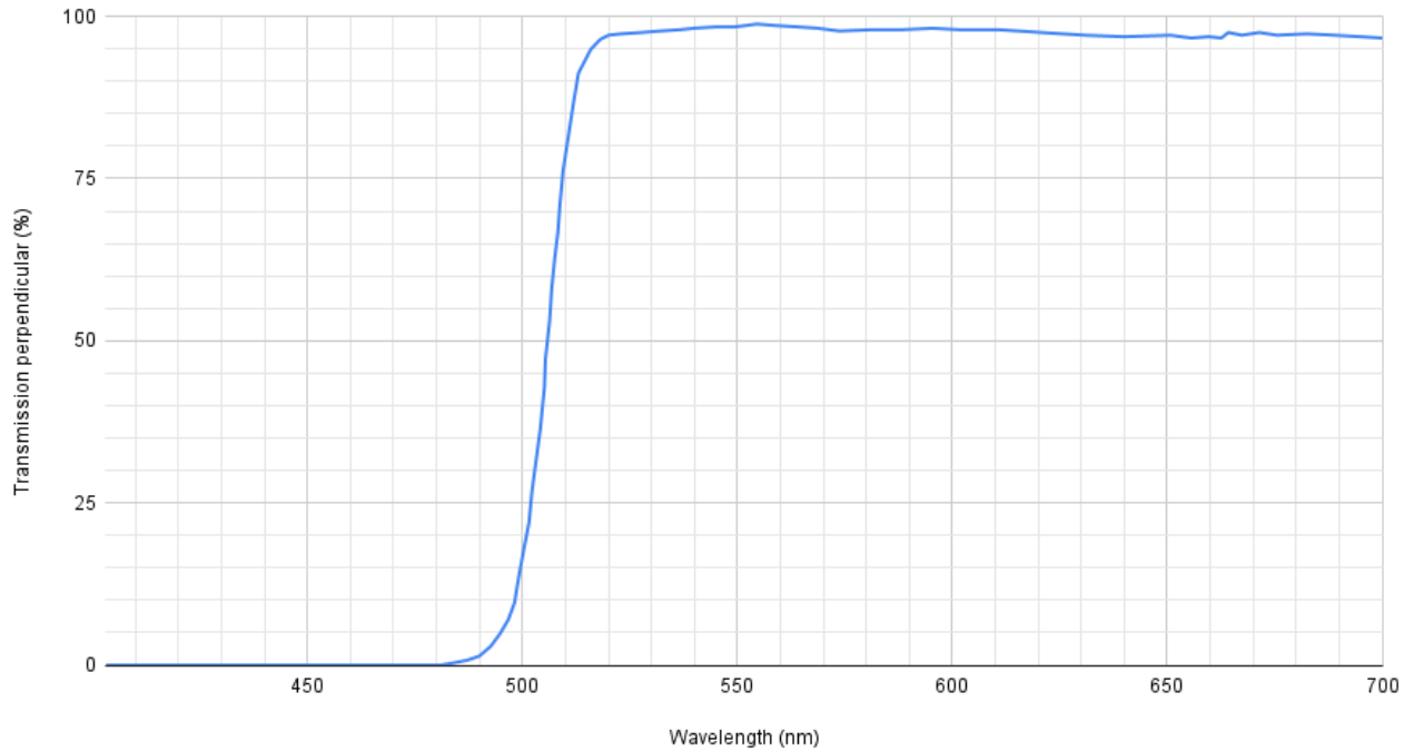
Dichroic Filter "refl. blue" (perpendicular, s)
