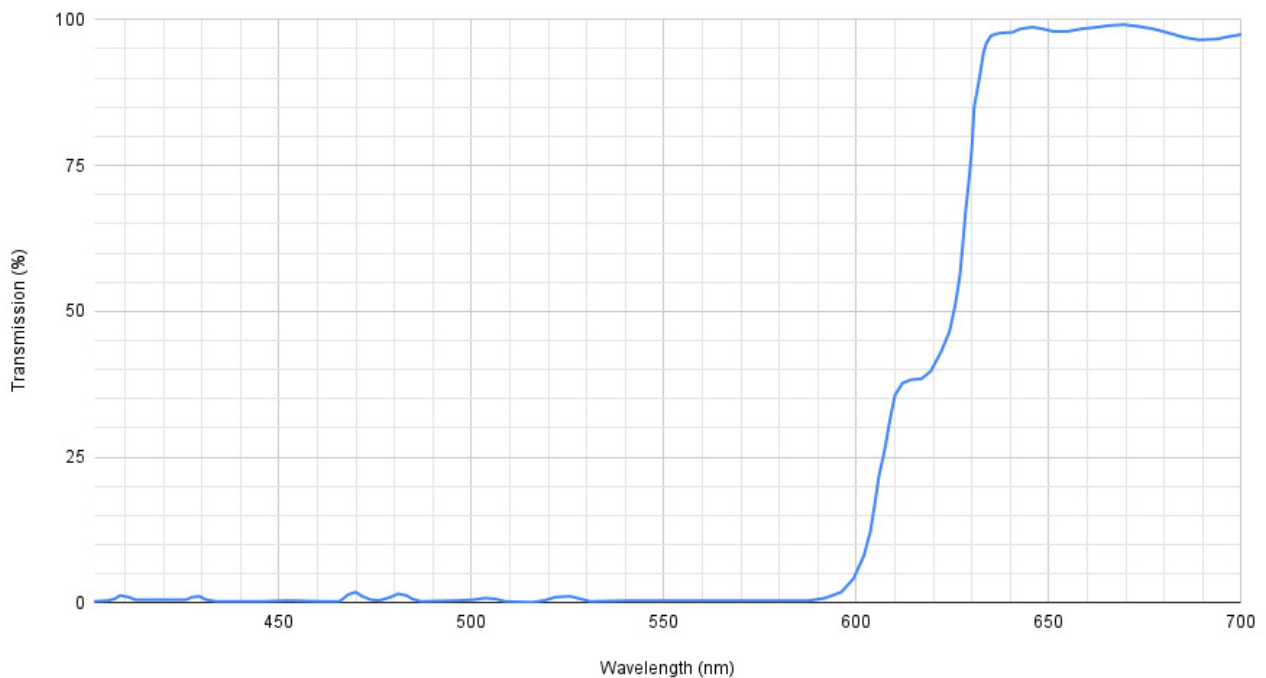
Dichroic Filter "LP600"
