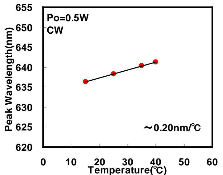
Peak Wavelength vs. Temperature
