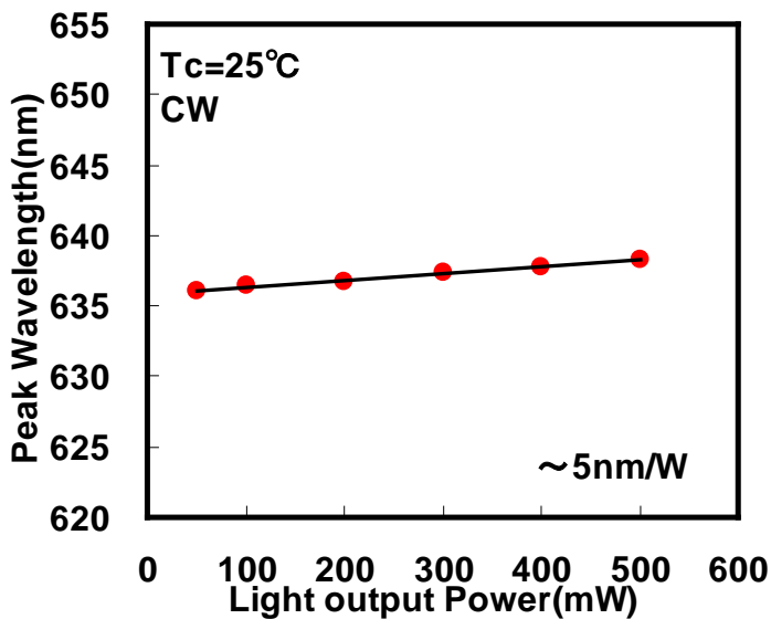
Peak Wavelength vs. Light Output Power
